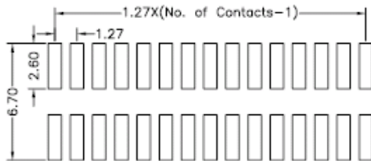
Recommended PCB Board Hole Layout
