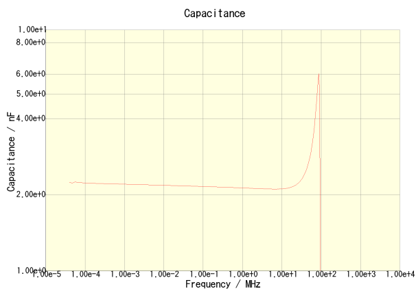
C3216X7R2J222K115AA
