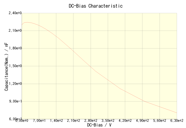
C3216X7R2J222K115AA
