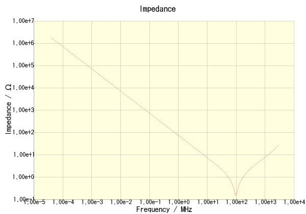
C3216X7R2J222K115AA
