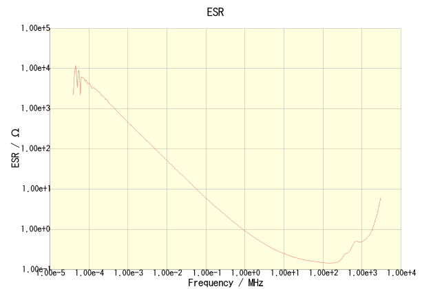
C3216X7R2J222K115AA
