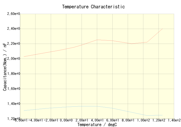
C3216X7R2J222K115AA(DC Bias = 0V) C3216X7R2J222K115AA(DC Bias = 315V)
