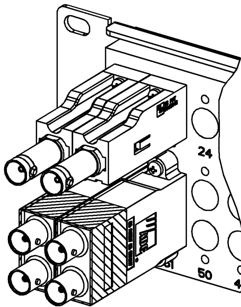
ISOMETRIC REAR VIEW (SHOWN SVJ JACKS AND CJ AS MON, 2 RU) SCALE 0.750
