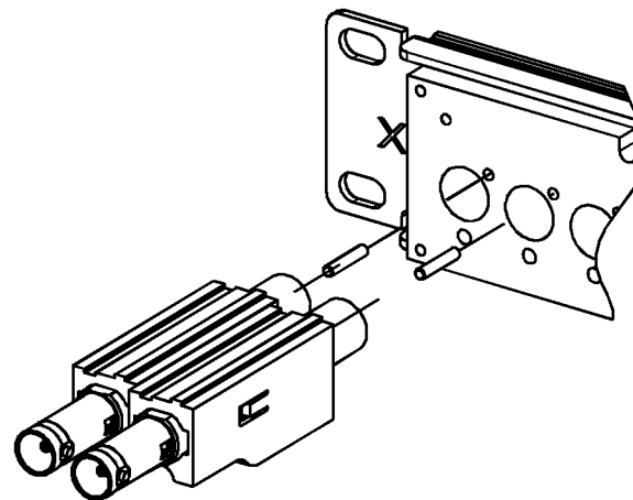
ISOMETRIC REAR VIEW (SHOWN 1 ROW CJ JACKS 1RU) SCALE 0.600
