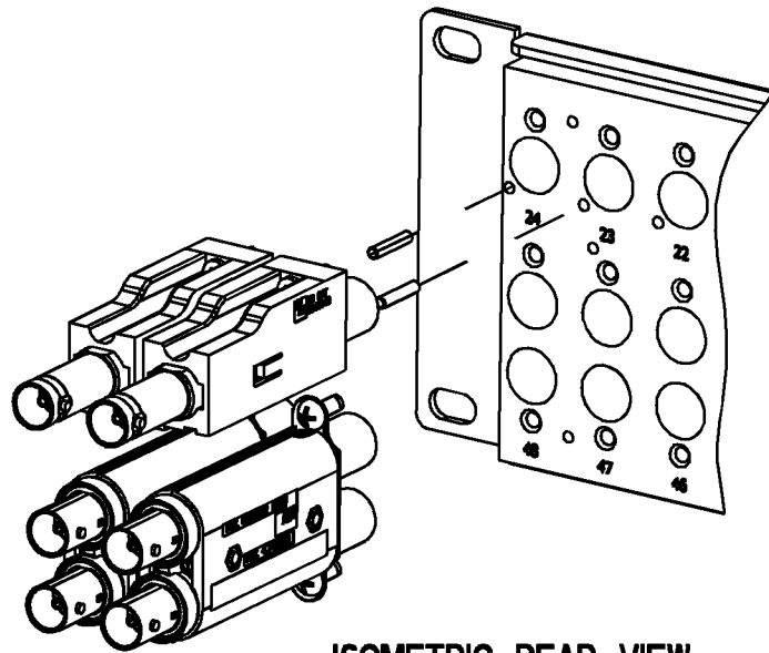
ISOMETRIC REAR VIEW (3 ROWS SJ JACKS AND CJ AS MON, 2RU) SCALE 0.600
