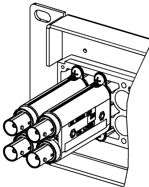
ISOMETRIC REAR VIEW (SHOWN N-JACKS, 2 RU) SCALE 0.750
