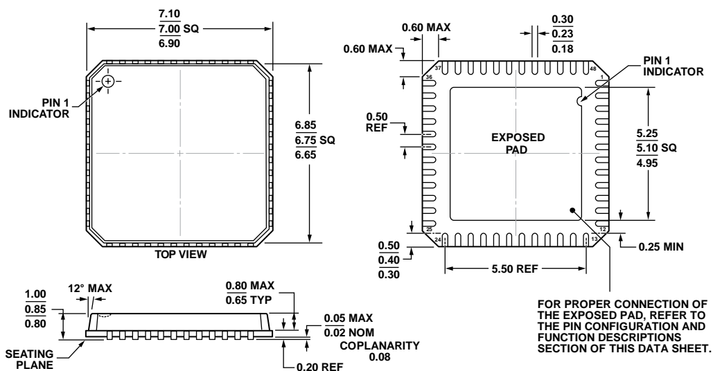
Dimensions shown in millimeters
