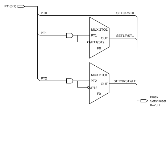
Figure 5. Set/Reset Generator
