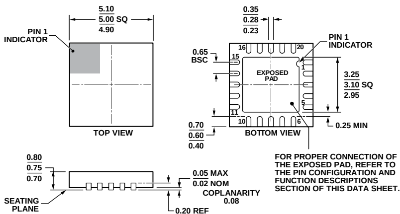
Figure 68. 20-Lead Lead Frame Chip Scale Package [LFCSP_WQ] 5 mm x 5 mm Body, Very Very Thin Quad (CP-20-9)
