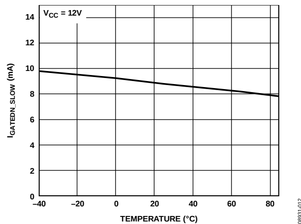
Figure 11. Gate Pull-Down Current ( I_{GATEDN\_SLOW} ) vs. Temperature
