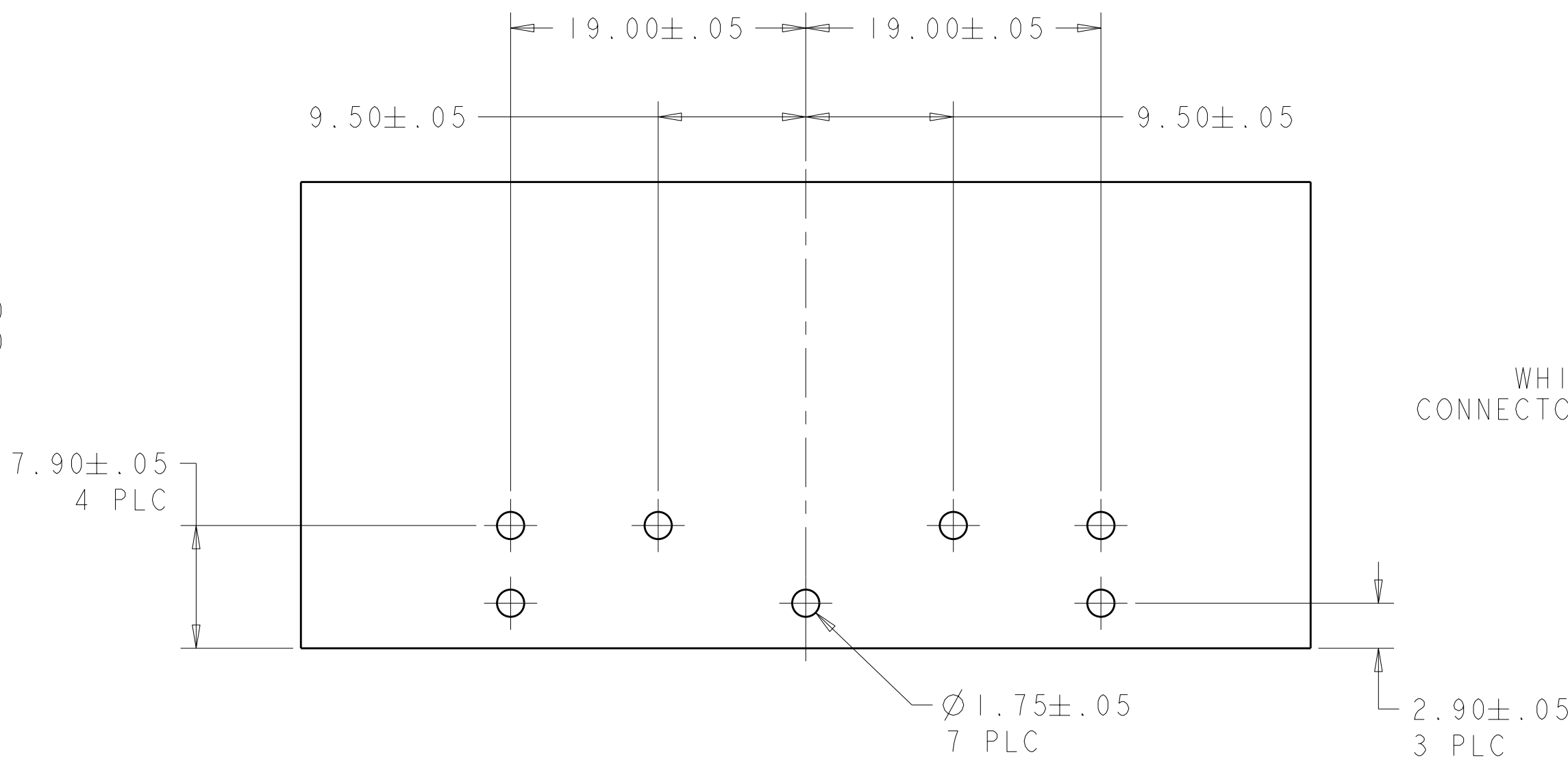
RECOMMENDED HOLE PATTERN SCALE 3:1
