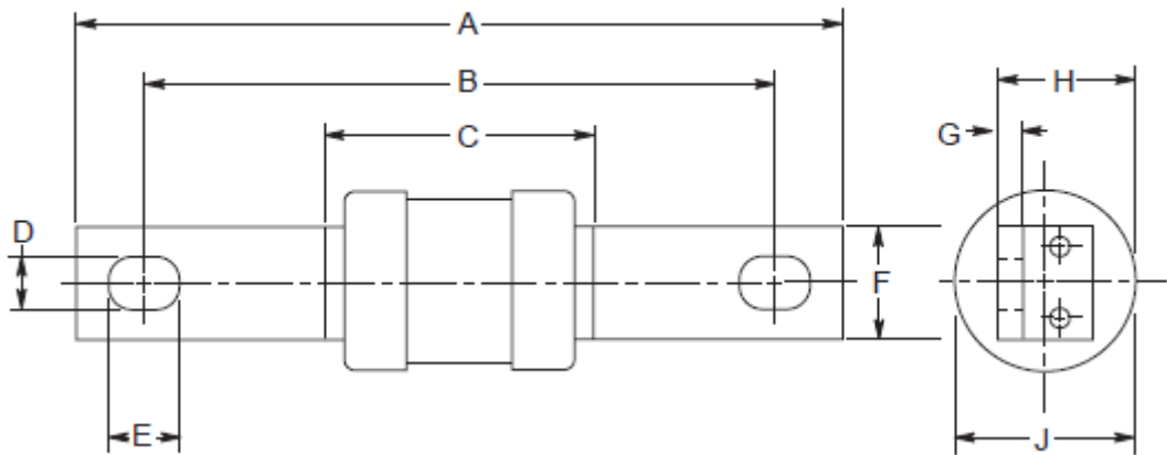
Dimensions - mm
