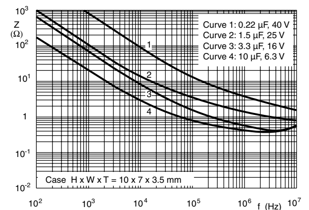
Fig.19 Typical impedance at 25 °C as a function of frequency
