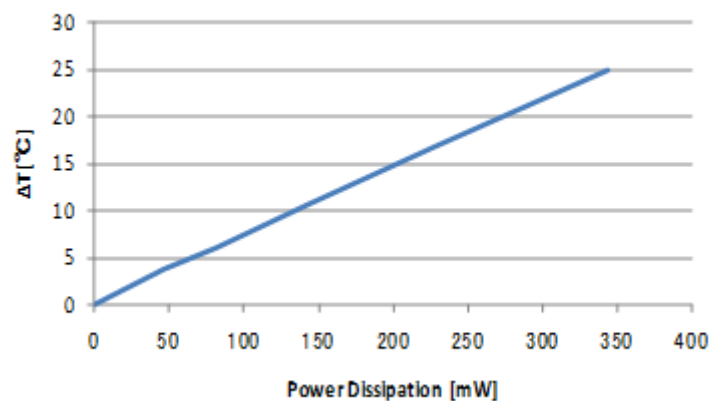
Loss - \Delta T Characteristics (Vin=3.6V, Vo=3.3V)
