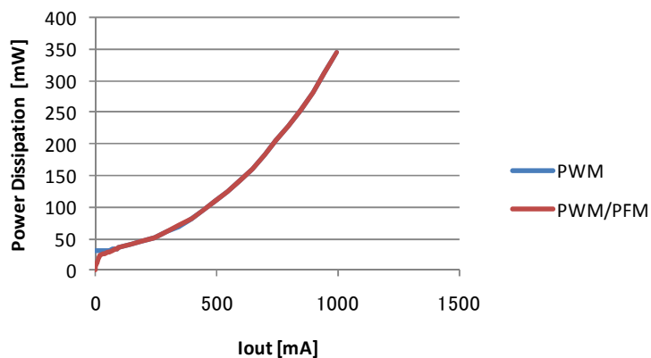
Io - Loss Characteristics (Vin=5.0V, Vo=3.3V)
