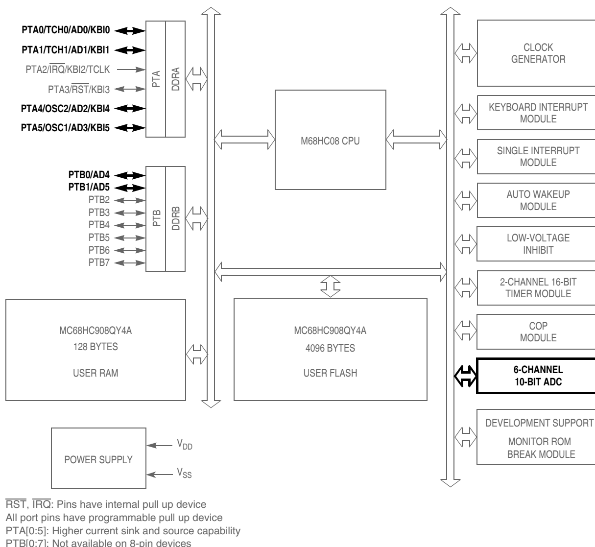
Figure 3-1. Block Diagram Highlighting ADC10 Block and Pins
