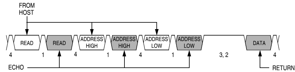
Figure 15-15. Read Transaction
