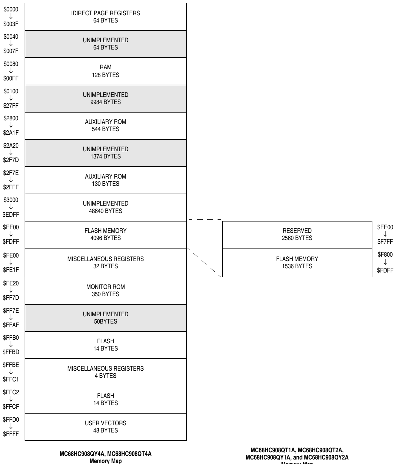
Figure 2-1. Memory Map
