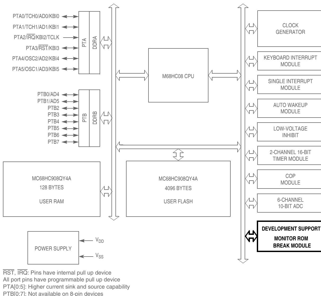
Figure 15-1. Block Diagram Highlighting BRK and MON Blocks
