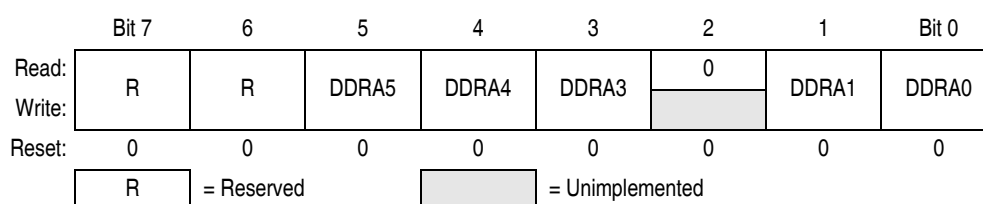
Figure 12-2. Data Direction Register A (DDRA)
