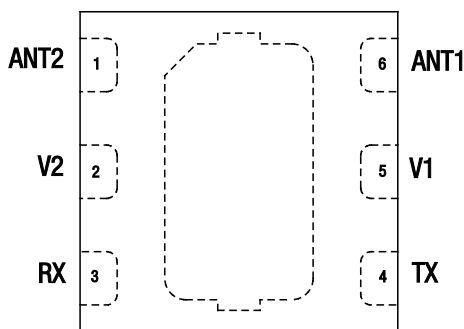
Figure 2. SKY13381-374LF Pinout – 6-Pin MLPD (Top View)
