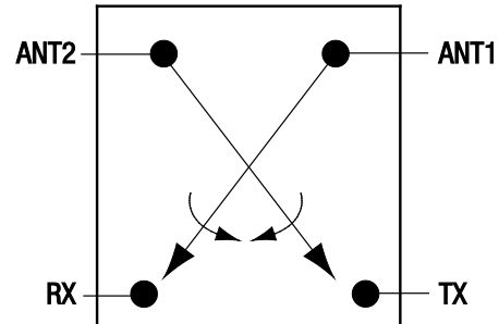
Figure 1. SKY13381-374LF Block Diagram
