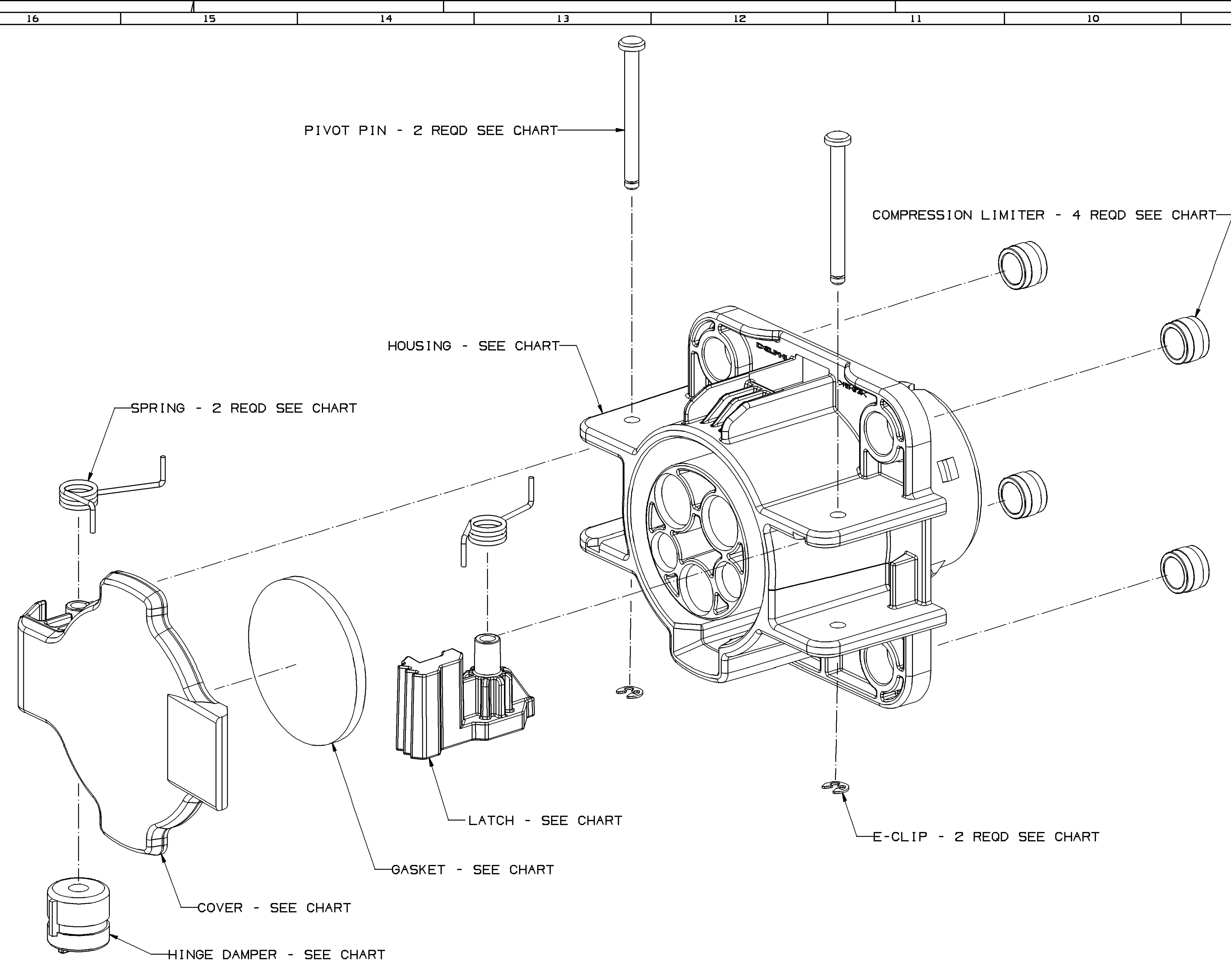
EXPLODED VIEW SCALE 2:1
