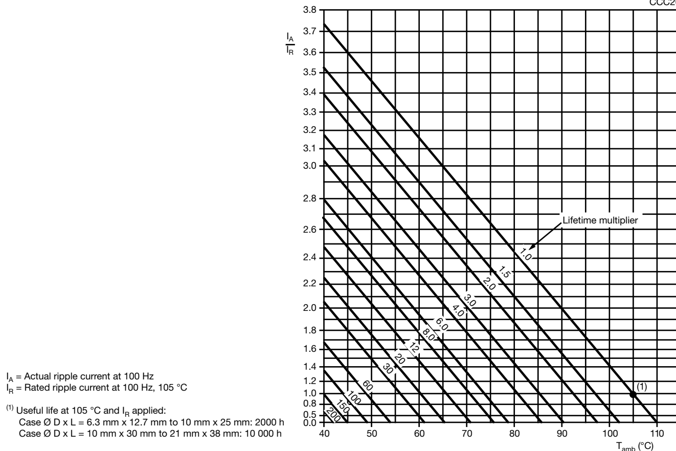
Fig. 19 - Multiplier of useful life as a function of ambient temperature and ripple current load
