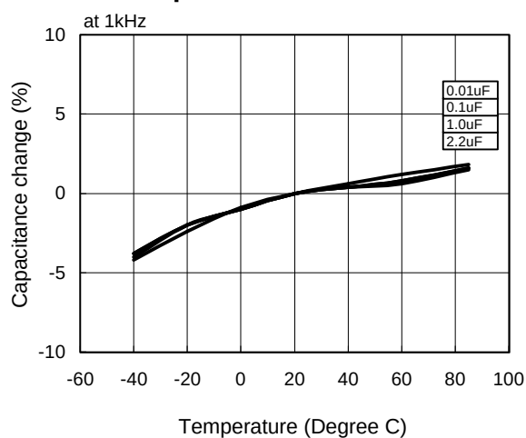
Temperature Characteristics
