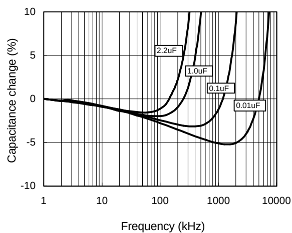
Frequency Characteristics
