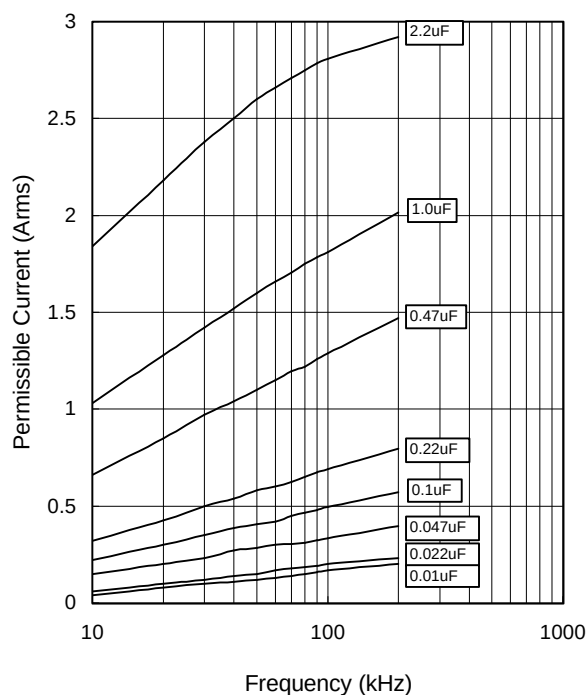
Permissible Current
