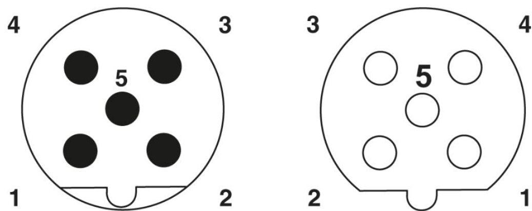
Pin assignment M12 male connector, 5-pos., B-coded, male side
