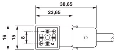
Dimensioned drawing
