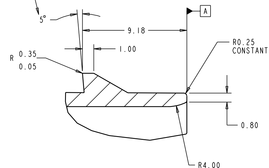
DETAIL A SCALE 8:1
