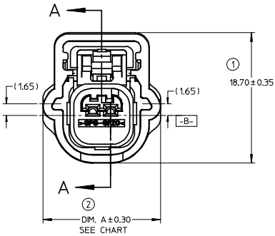
FRONT VIEW POLARIZATION A
