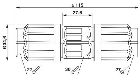
QPD C 5x2.5 dimensional drawing
