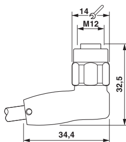
Dimensioned drawing
