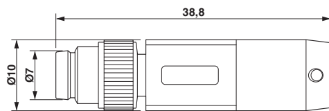
Dimensioned drawing
