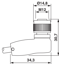
Dimensioned drawing
