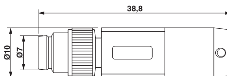
Dimensioned drawing
