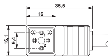
Dimensioned drawing
