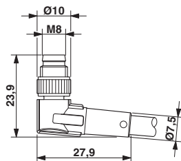
Dimensioned drawing
