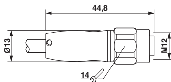
Dimensioned drawing
