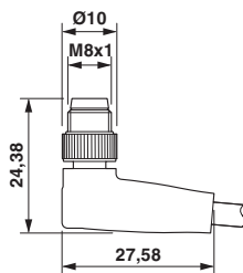
Dimensioned drawing
