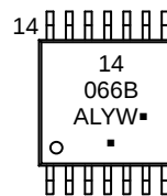
TSSOP-14
