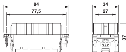
Dimensioned drawing
