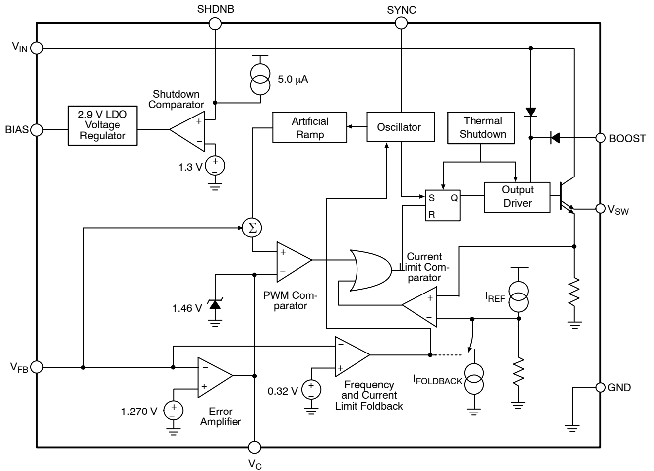
Figure 2. Block Diagram
