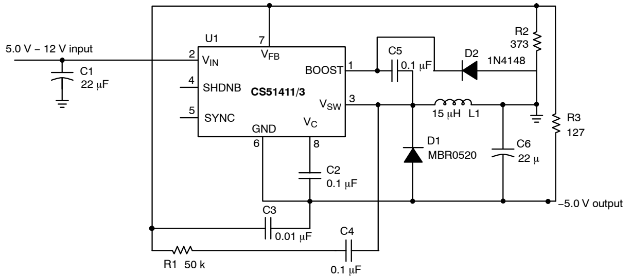
Figure 25. Additional Application Diagram, 5.0 V – 12 V to –5.0 V/400 mA Inverting Converter
