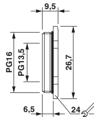
Dimensional drawing
