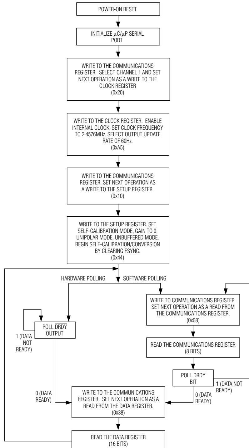
Figure 11. Sample Flow Diagram for Data Conversion
