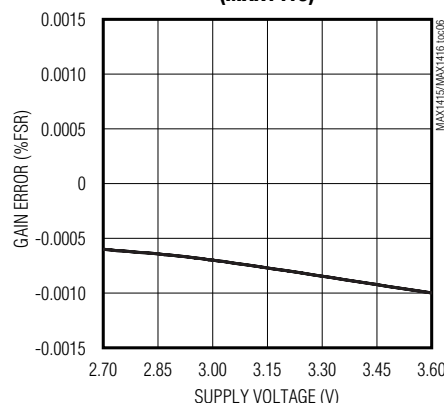
GAIN ERROR vs. SUPPLY VOLTAGE (MAX1415)
