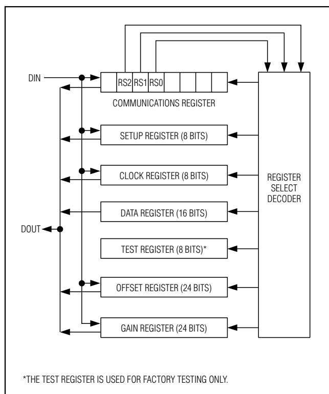
Figure 10. Register Summary
