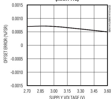
OFFSET ERROR vs. SUPPLY VOLTAGE (MAX1415)
