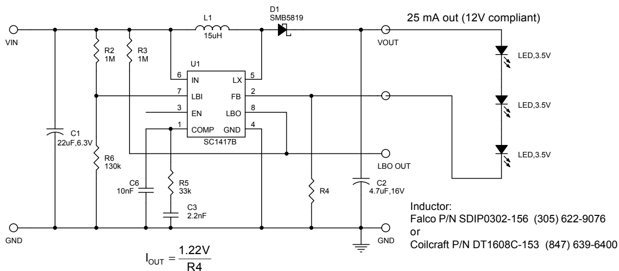
Figure 1 - Constant Brightness LED driver with 12V compliance from 2-cells (constant current output)
