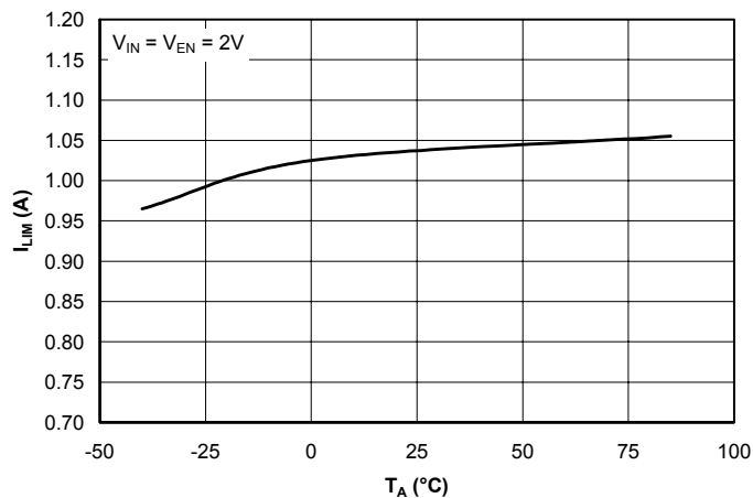
Power Switch Current Limit
