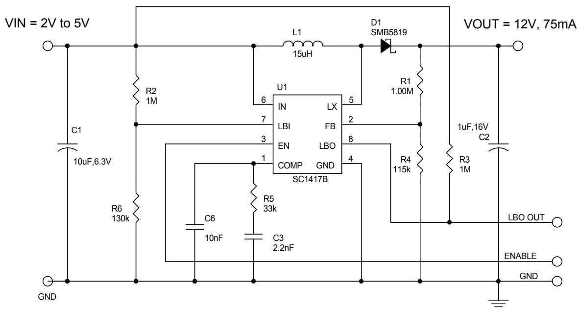
Figure 2 - Minimum Capacitance Boost Converter
