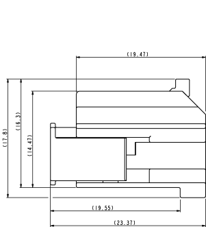
ASSEMBLY WITHOUT CPA
