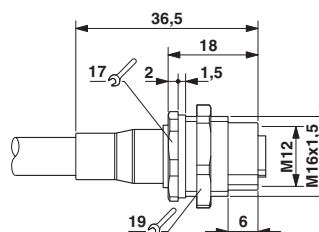
Dimensioned drawing
