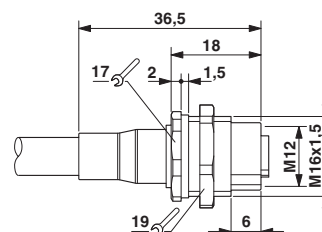
Dimensioned drawing
