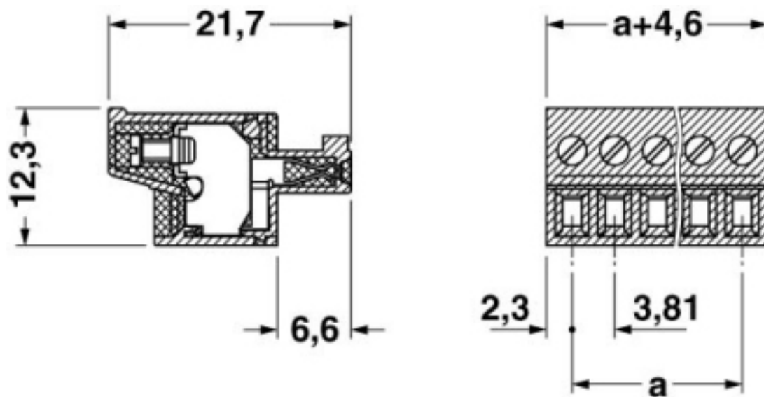
Dimensioned drawing
