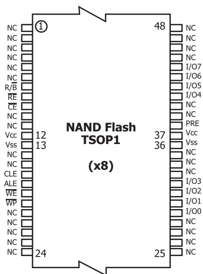
Figure 2. 48TSOP1 Contactations, x8 Device
