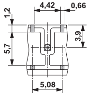
Dimensioned drawing
