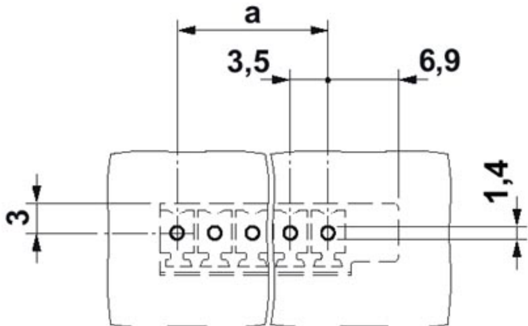
Drilling diagram
