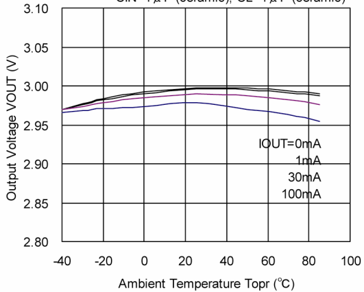
XC6219/11x302
