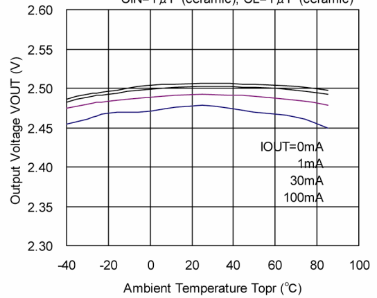
XC6219/11x252
