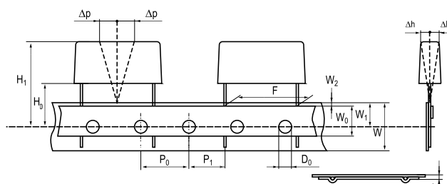
Lead Spacing 22.5 – 27.5 mm
