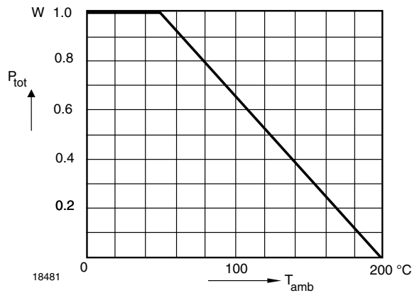
Figure 1. Admissible Power Dissipation vs. Ambient Temperature
