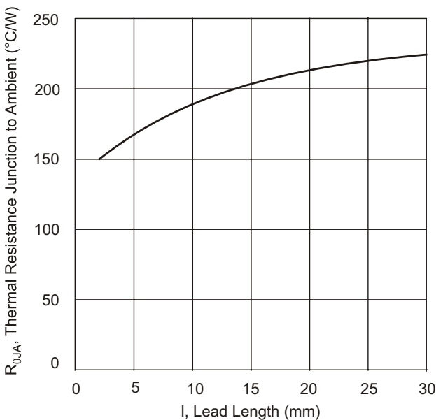
Fig. 2 Typical Thermal Resistance vs. Lead Length
