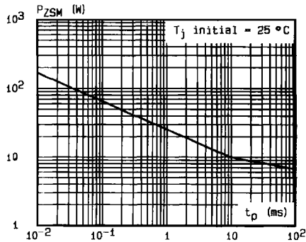
Fig.8 - Peak pulse power versus pulse duration (rectangular wave form).
