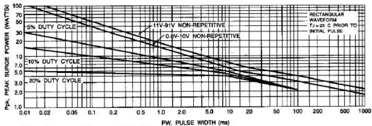
Fig. 5-MAXIMUM SURGE POWER
