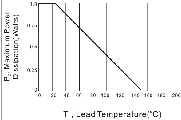
Fig.1 Steady-State Power Derating Curve
