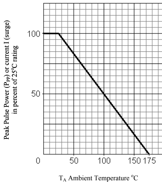
FIG. 4 Derating Curve
