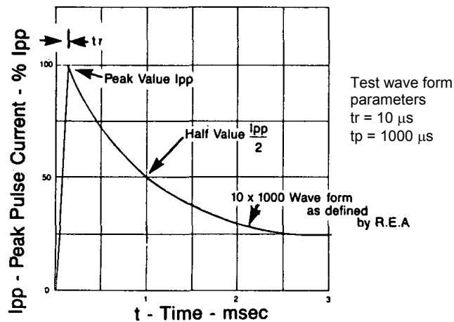
FIGURE 3 PULSE WAVEFORM
