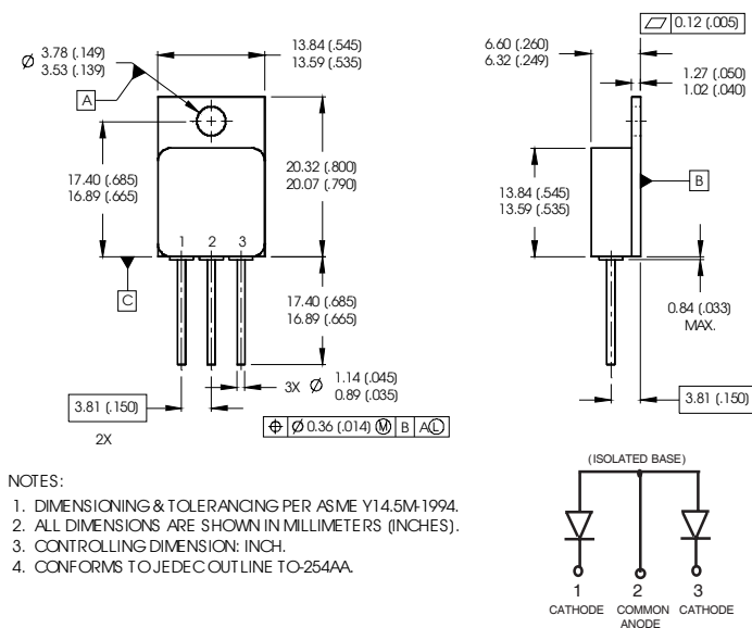
Case Outline and Dimensions - TO-254AA
